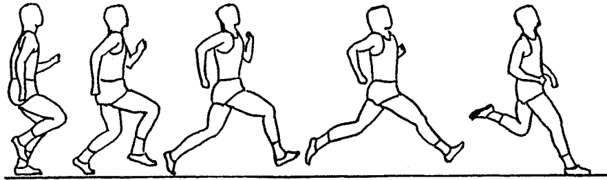
Figure 3: Final preparation for take-off during the last stride, shown from the swing leg squat up to the board contact phase (from left to right)
